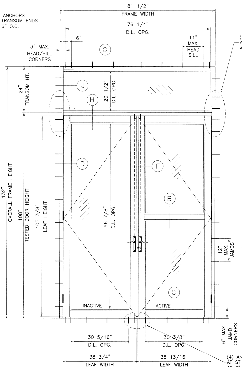
TYPICAL ELEVATION
