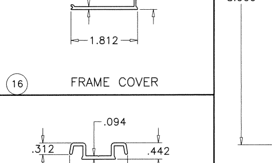
16 FRAME COVER
