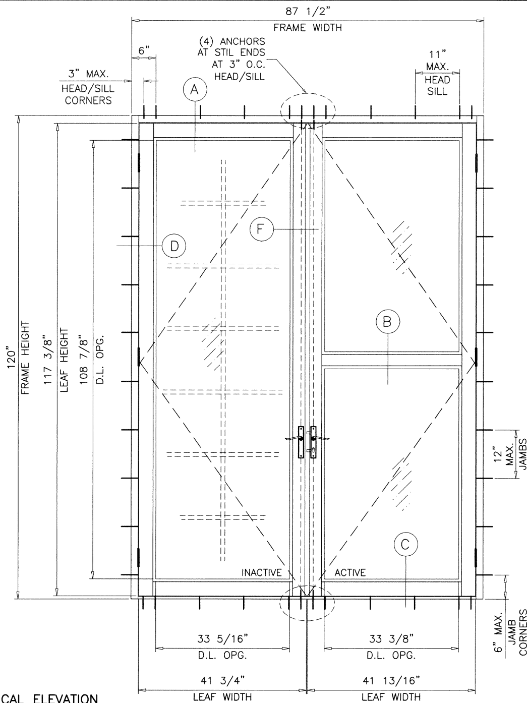
TYPICAL ELEVATION
