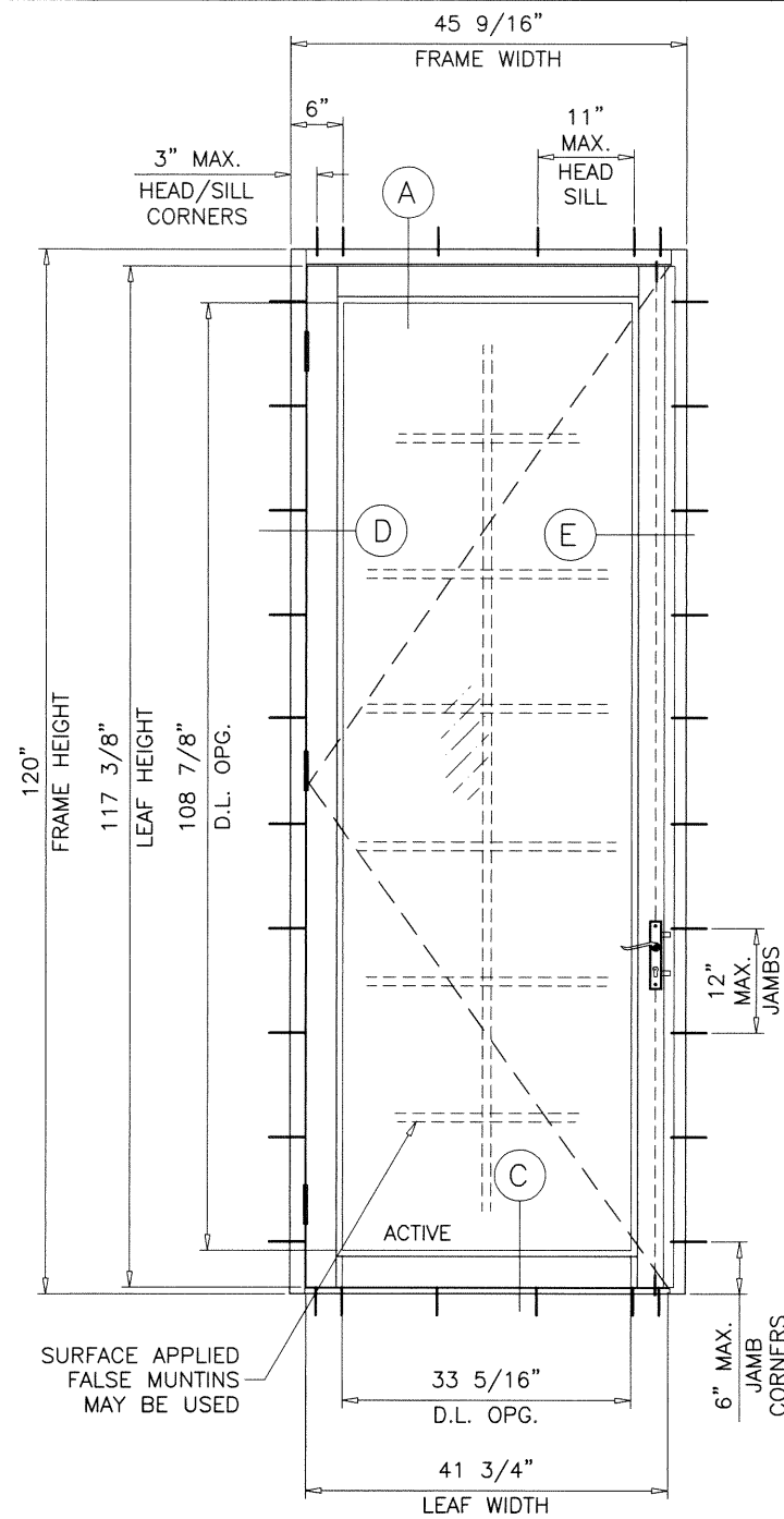
TYPICAL ELEVATION
