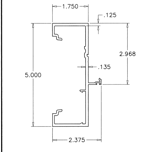
7 SHEAR CLIP
