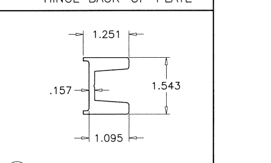
19 LEAF CLAMP HINGE BACK-UP PLATE
