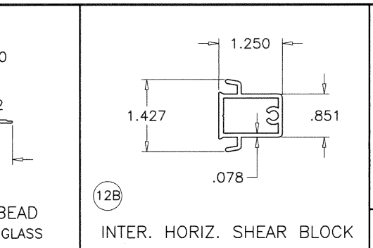
12B INTER. HORIZ. SHEAR BLOCK
