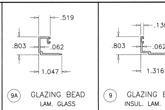
9A GLAZING BEAD LAM. GLASS
