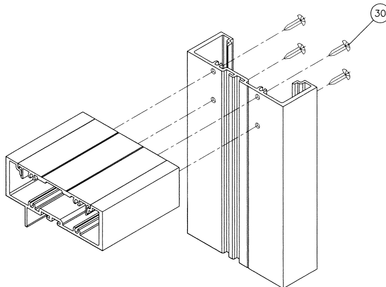
TRANSOM TOP CORNER
