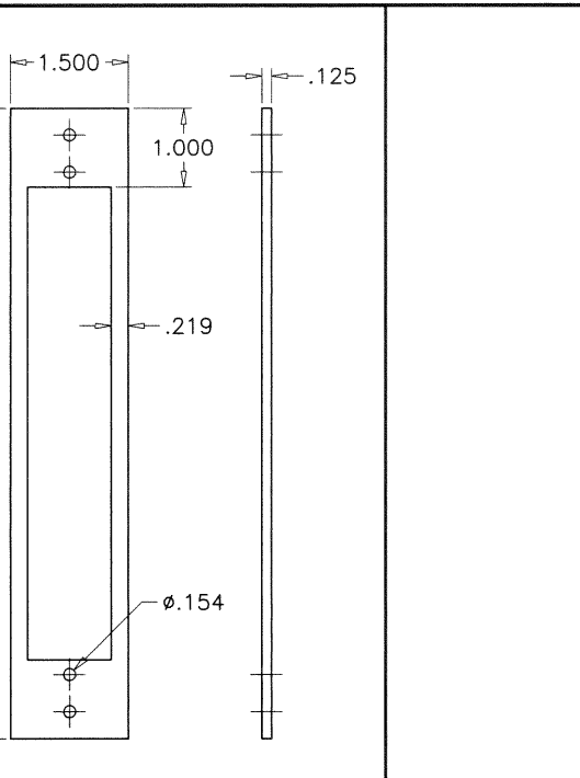
15 LOCK BACK-UP PLATE
