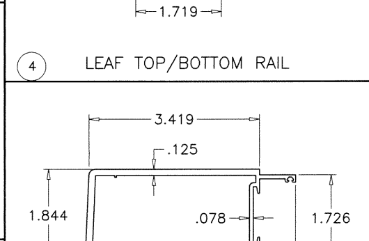
4 LEAF TOP/BOTTOM RAIL
