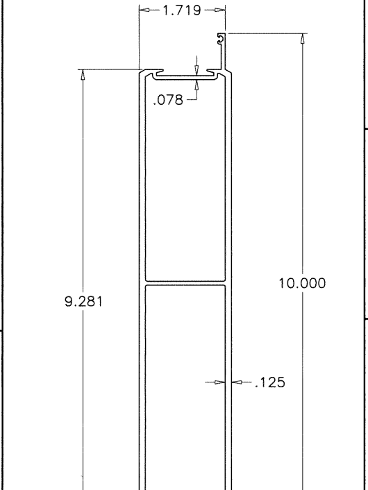
4A 10" BOTTOM RAIL
